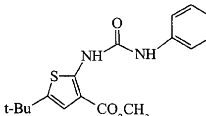
5-tert-Butyl-2-(3-phenyl-ureido)-thiophene-3-carboxylic acid methyl ester
